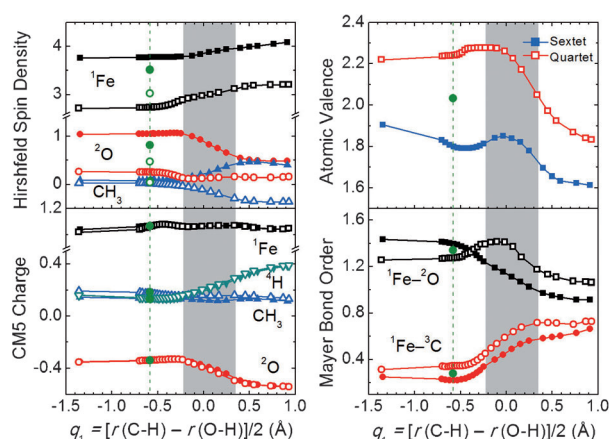
Figure 5. Hirshfeld spin densities, CM5 partial charges, atomic valences of Fe, and Mayer bond orders along the HAT coordinate. The C–H bond breaking and O–H bond formation occurred rapidly in the shaded region with very little heavy atom motion. The closed and open symbols represent sextet and quartet spin states, respectively. The green dashed lines and points represent the positions and individual values of the MECP, respectively.
